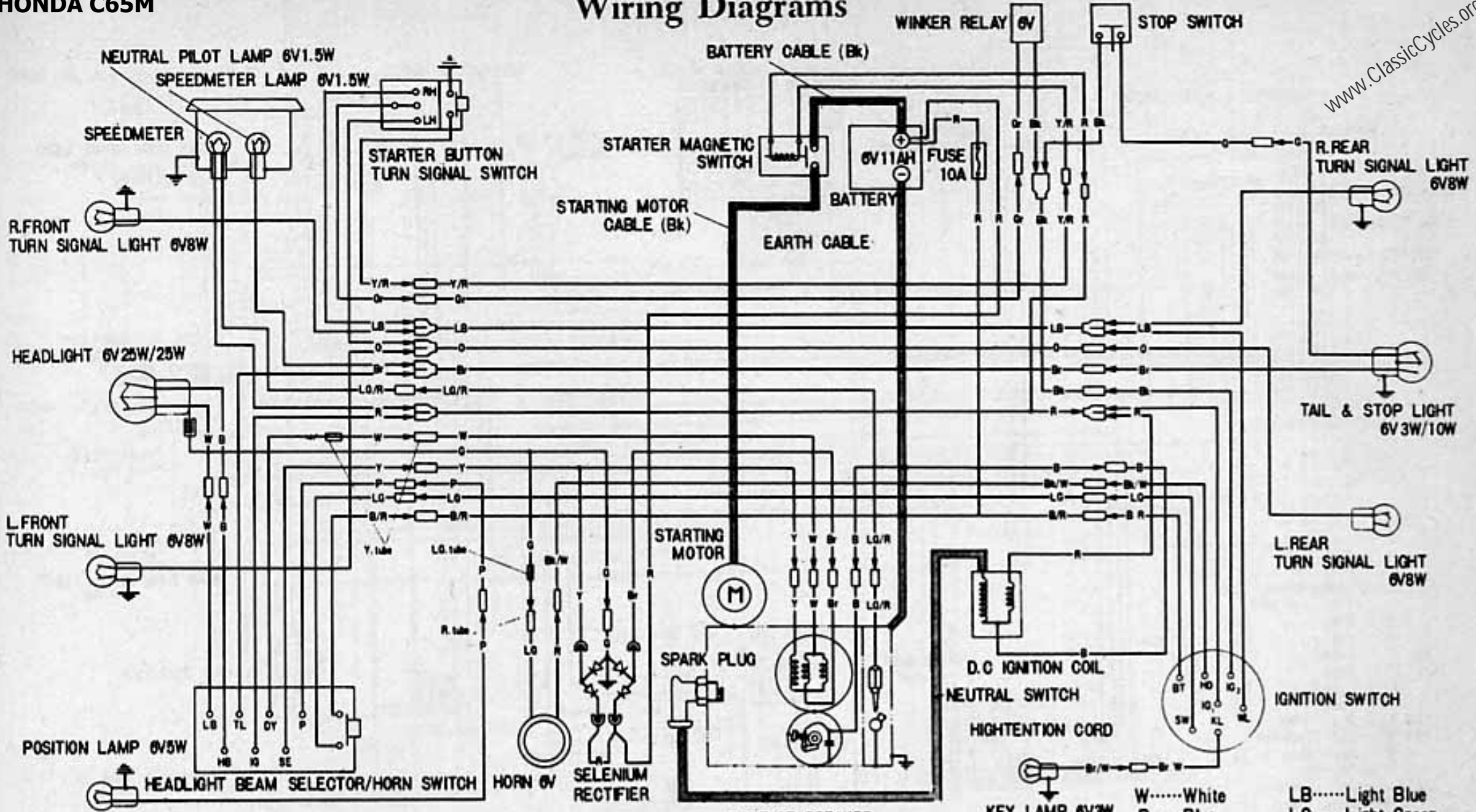
HEADLIGHT BEAM SELECTOR SWITCHING ARRANGEMENT
